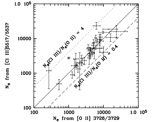
Fig. 9. Same as Fig. 8 but for densities derived from the [Cl III] and [O II] doublet ratios, respectively.
